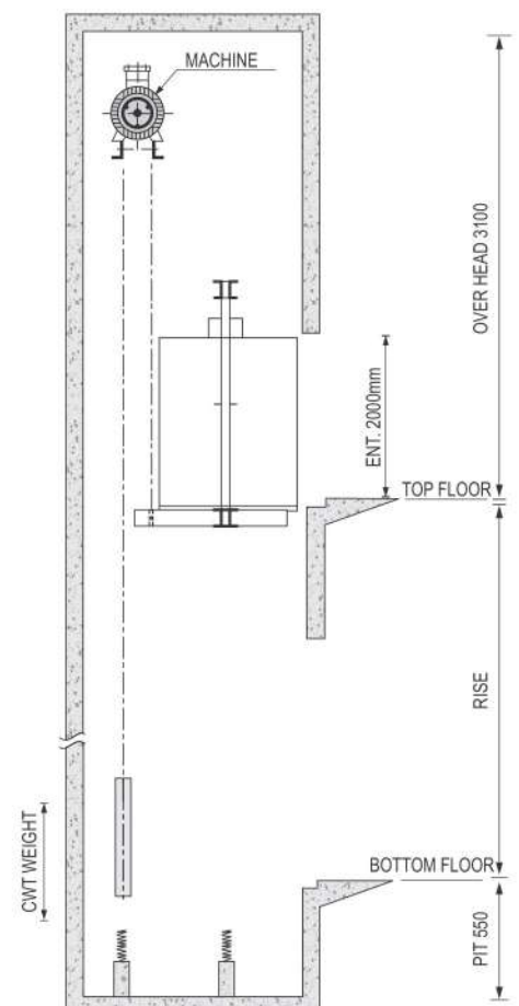
HOISTWAY ELEVATION PLAN
